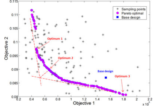
Fig. 12. Pareto-solutions of multiple-objective optimization.
