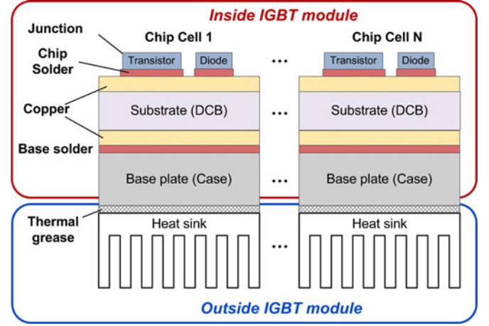
Fig. 2. IGBT physical structure with multicells.
