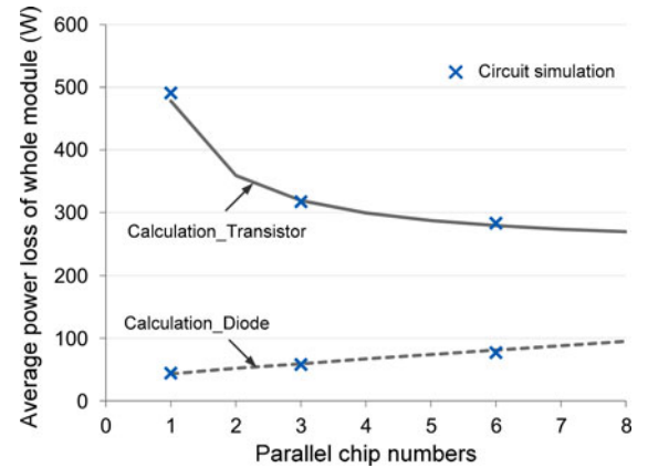
Fig. 22. Comparison of power loss by circuit simulation and model calculation under different chip numbers (conditions in Table I, switching energy in Fig. 17 is used, T_c = 80^\circ\text{C} ).
