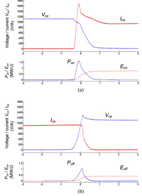
Fig. 16. Experimental switching waveforms of IGBT with corresponding free-wheeling diode (IGBT module 1700 V/1000 A, T_j = 125^\circ \text{C} , V_{dc} \approx 1120 \text{ V} , I_c \approx 940 \text{ A} ). (a) Transistor turning ON, (b) Transistor turning OFF.
