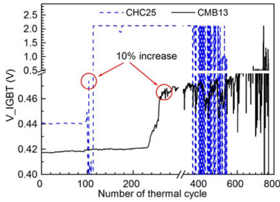
Fig. 18. Evolutions of on-state voltage drops, V_{IGBT} s, across the IGBTs in the samples CHC and CMB13 at 90 °C, with respect to number of thermal cycle between -55 and 150 °C.
