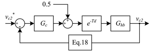
Fig. 7. Control block diagram for the proposed active power decoupling circuit.
