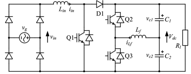
Fig. 2. Proposed symmetrical half-bridge circuit for single-phase active power decoupling.
