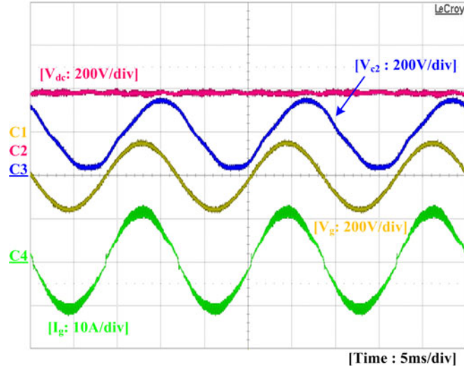
Fig. 10. Steady-state experimental waveforms with ripple power compensation. From top to bottom, dc-link voltage, lower capacitor voltage, grid voltage, and grid current.
