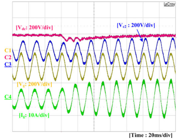
Fig. 13. Dynamic experimental waveforms showing 50% to 100% step-up load change. From top to bottom, dc-link voltage, lower capacitor voltage, grid voltage, and grid current.
