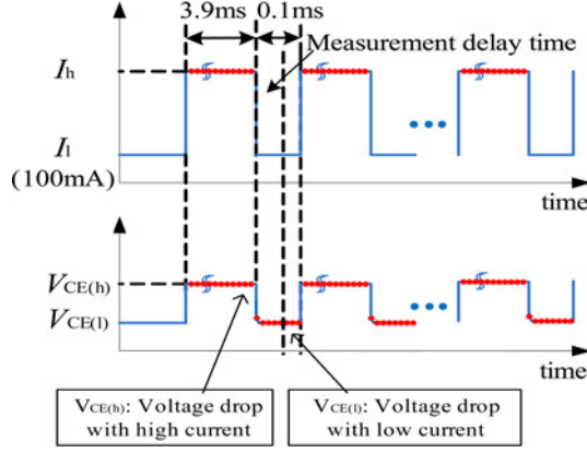
Fig. 3. Train of current pulses for solder D&amp;P tests.
