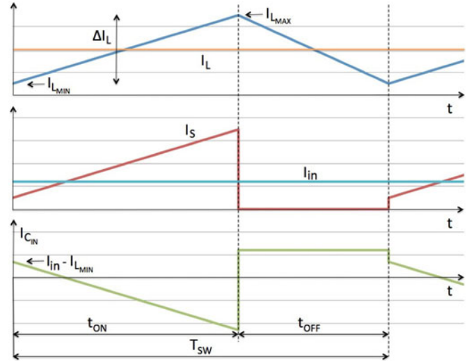
Fig. 8. Plots of the currents in a Buck or Buck-Boost derived converter without M_{cap} (values are generic): in the inductor ( I_L blue, and I_{L,AVG} orange); in the switch ( I_S red) and average input current ( I_{in} light blue); in the input capacitor ( I_{C_{in}} green).
