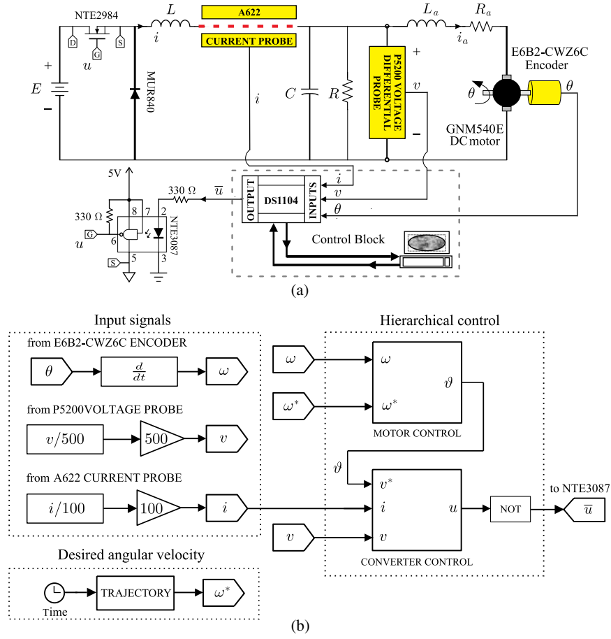
Fig. 4. Connections and synthesis of the control to accomplish the experimental results. (a) Diagram of connections. (b) Control block developed in MATLAB-Simulink.
