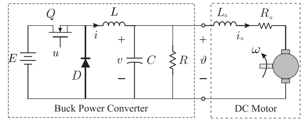
Fig. 1. DC/DC Buck power converter–dc motor system.
