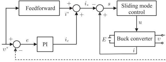
Fig. 2. Cascade control for the Buck power converter.
