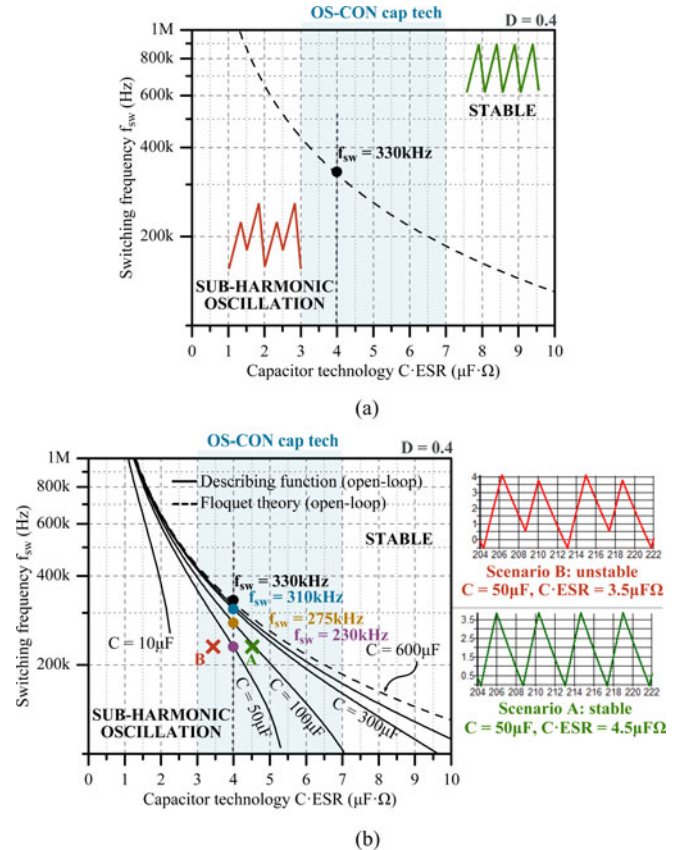
Fig. 7. Stability condition of constant frequency V^2 peak control and being the slow loop open using (a) DF and (b) Floquet theory. On the right of (b), the inductor current waveforms for an unstable case and a stable case are shown. (a) Stability condition from DF. (b) Comparison between DF and the Floquet theory.
