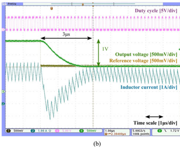
Fig. 17. Experimental validation of discrete modeling under a voltage reference step 2\text{ V} \rightarrow 1\text{ V} . (a) Discrete modeling. (b) Experimental prototype.
