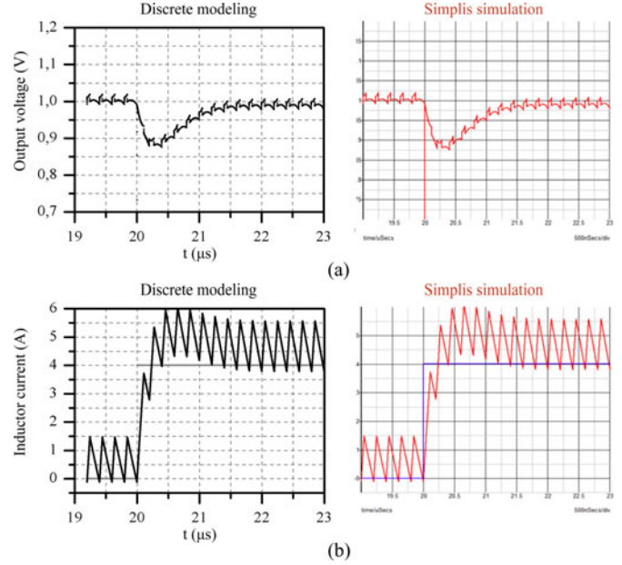
Fig. 11. Comparison between the discrete model (left) and simulation results (right) under a load step 0 \text{ A} \rightarrow 4 \text{ A} . (a) Output voltage. (b) Inductor current.
