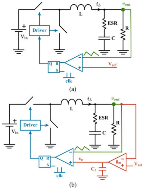
Fig. 6. Control scheme of a constant-frequency V^2 peak control. (a) V^2 with the slow loop opened. (b) V^2 with the slow loop closed for precise regulation of the output voltage.
