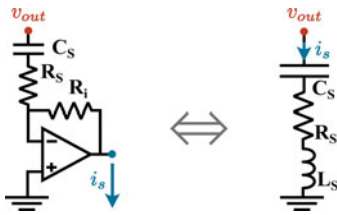
Fig. 4. Current sensor behaves like a RLC network.
