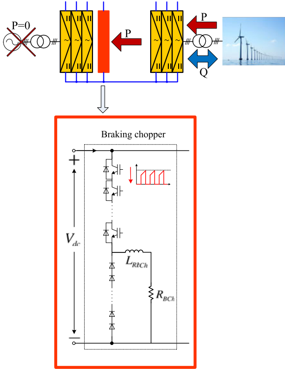
Fig. 8. Conventional braking chopper circuit.
