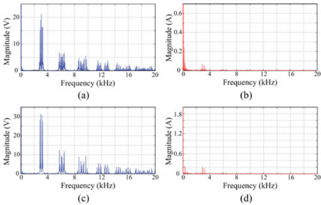
Fig. 12. Measured harmonic spectrums of half-bridge MMC when applying the circulating current harmonics cancellation PSC-PWM: (a) phase voltage u_{0a} , (b) circulating current i_{ca} , (c) line-to-line voltage u_{ab} , and (d) dc-link current i_{dc} .
