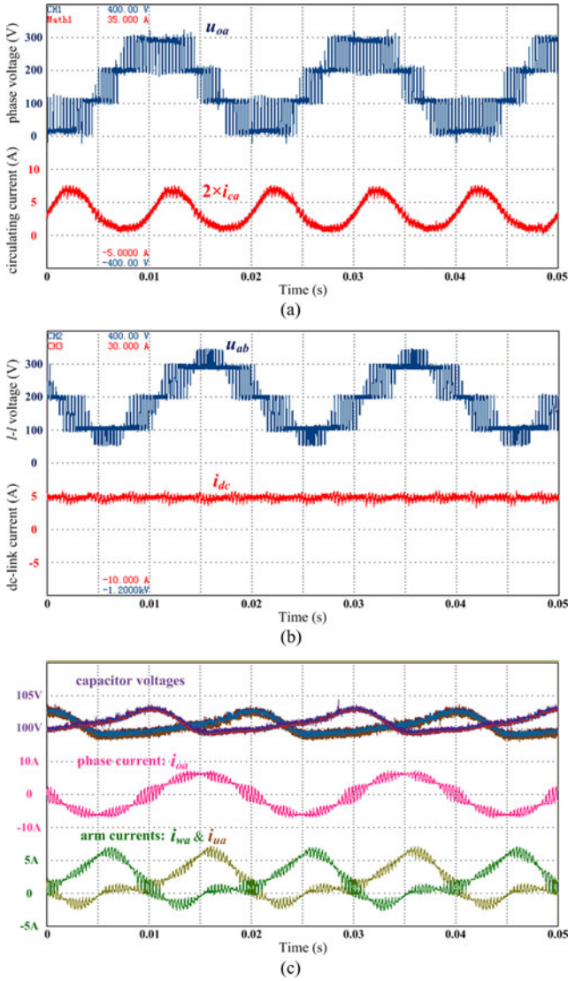
Fig. 11. Experimental waveforms of half-bridge MMC when applying the circulating current harmonics cancellation PSC-PWM: (a) phase voltage u_{0a} and circulating current i_{ca} , (b) line-to-line voltage u_{ab} and dc-link current i_{dc} , (c) SM capacitor voltages of phase a , phase current i_{0a} , lower arm current i_{wa} , and upper arm current i_{ua} .
