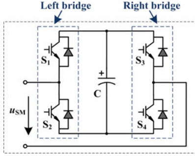
Fig. 7. Configuration of a full-bridge SM.
