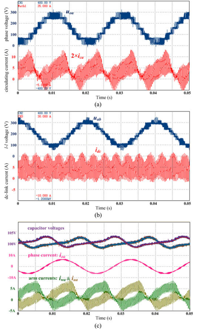
Fig. 13. Experimental waveforms of half-bridge MMC when applying the output voltage harmonics minimization PSC-PWM: (a) phase voltage u_{0a} and circulating current i_{ca} , (b) line-to-line voltage u_{ab} and dc-link current i_{dc} , (c) SM capacitor voltages of phase a , phase current i_{0a} , lower arm current i_{wa} , and upper arm current i_{ua} .
