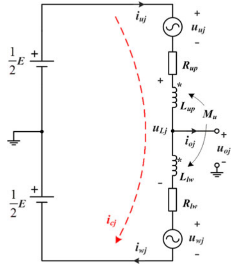
Fig. 2. Equivalent circuit of one phase of the MMC.
