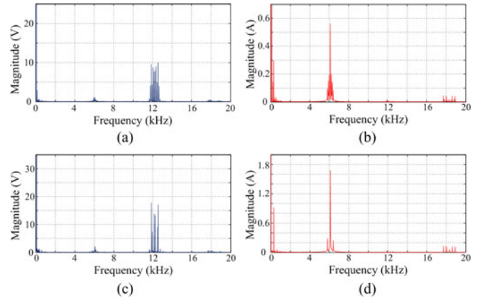
Fig. 18. Measured harmonic spectrums of full-bridge MMC when applying the output voltage harmonics minimization PSC-PWM: (a) phase voltage u_{0a} , (b) circulating current i_{ca} , (c) line-to-line voltage u_{ab} , (d) dc-link current i_{dc} .
