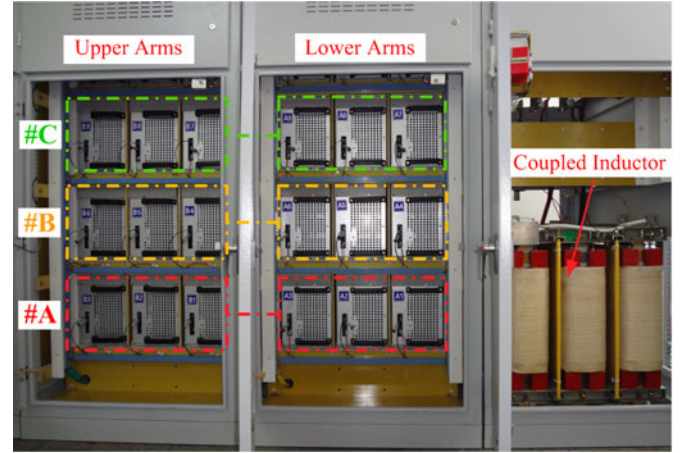
Fig. 9. Laboratory setup.
