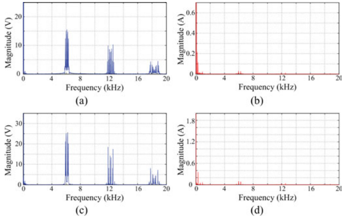
Fig. 16. Measured harmonic spectrums of full-bridge MMC when applying the circulating current harmonics cancellation PSC-PWM: (a) phase voltage u_{0a} , (b) circulating current i_{ca} , (c) line-to-line voltage u_{ab} , (d) dc-link current i_{dc} .
