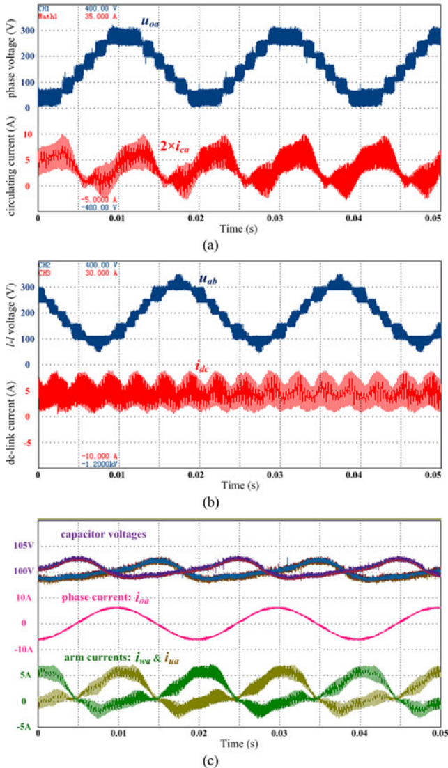
Fig. 17. Experimental waveforms of full-bridge MMC when applying the output voltage harmonics minimization PSC-PWM: (a) phase voltage u_{0a} and circulating current i_{ca} , (b) line-to-line voltage u_{ab} and dc-link current i_{dc} , (c) SM capacitor voltages of phase a , phase current i_{0a} , lower arm current i_{wa} , and upper arm current i_{ua} .
