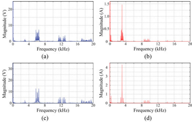
Fig. 14. Measured harmonic spectrums of half-bridge MMC when applying the output voltage harmonics minimization PSC-PWM: (a) phase voltage u_{oa} , (b) circulating current i_{ca} , (c) line-to-line voltage u_{ab} , (d) dc-link current i_{dc} .
